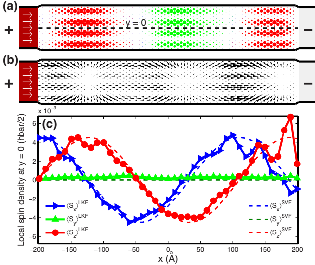
FIG. 3. (Color online) Local spin density of (a) the out-of-plane component \langle S_z \rangle and (b) the in-plane component (\langle S_x \rangle, \langle S_y \rangle) in a conducting sample made of Au(111) surface, subject to a ferromagnetic source lead with +x magnetization. (c) \langle S_x \rangle , \langle S_y \rangle , and \langle S_z \rangle as a function of x at y=0 , i.e., along the dashed line sketched in (a). Computed values are compared with the previously obtained spin vector formula based on quantum mechanics.
