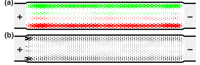
FIG. 2. (Color online) Local spin density of (a) the out-of-plane component \langle S_z \rangle and (b) the in-plane component \langle S_x \rangle, \langle S_y \rangle in a 398.9 \times 63.3 (total number of sites N=931 ) conducting sample made of Au(111) surface. The size of each local marker depicts the magnitude. In (a), red/dark (green/light) dots denote \langle S_z \rangle > 0 ( \langle S_z \rangle < 0 ). The maximum of \langle S_z \rangle is 1.2 \times 10^{-3}(\hbar/2) while the mean of \langle S_y \rangle is 3.16 \times 10^{-4}(\hbar/2) .
