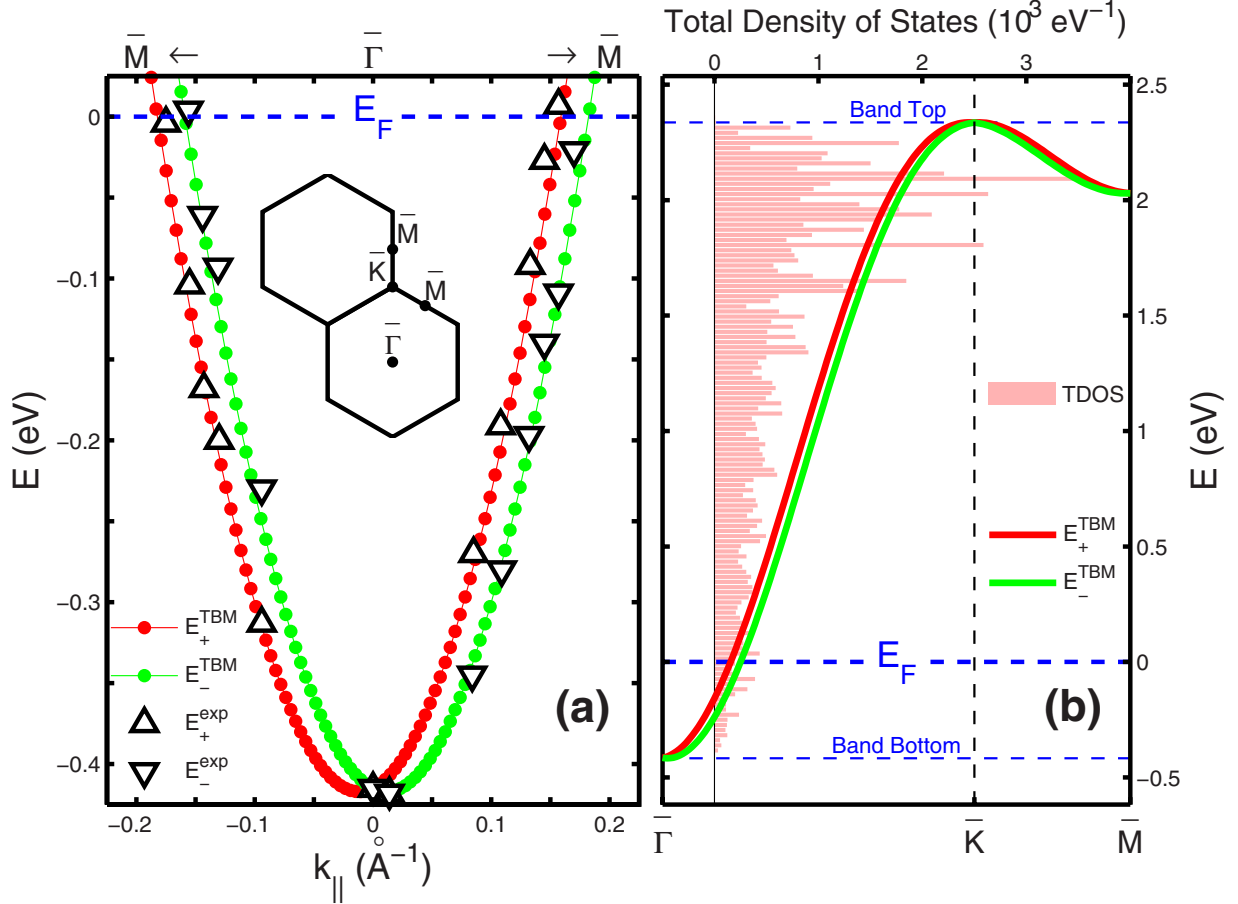
FIG. 1. (Color online) (a) Tight-binding energy dispersion E_{\pm}^{\text{TBM}} and the experimentally measured binding energy E_{\pm}^{\text{exp}} of Ref. 11 along the \bar{\Gamma}\bar{M} direction. The surface Brillouin zone is sketched in the inset. (b) Total density of states and E_{\pm}^{\text{TBM}} along \bar{\Gamma}\bar{K} and \bar{K}\bar{M} directions.
